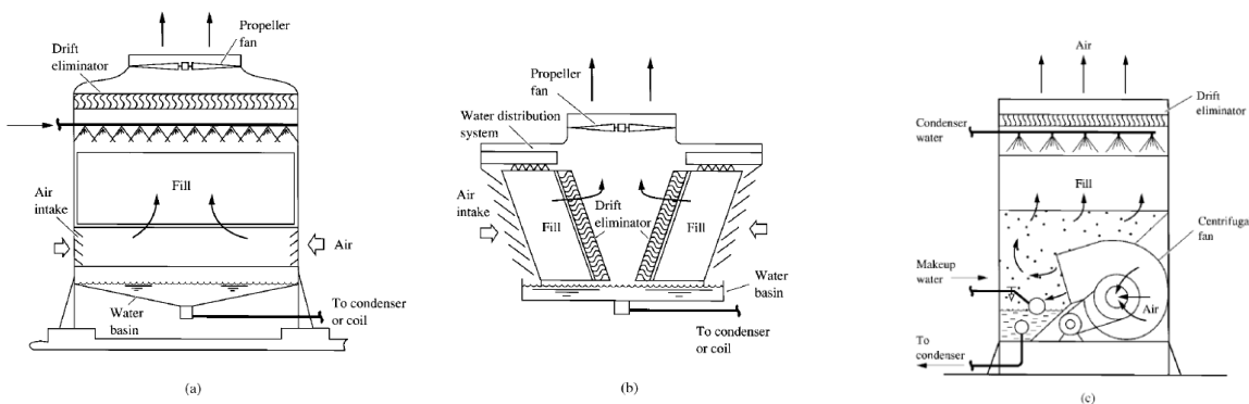
FIGURE 2 Type of Cooling Towers.
